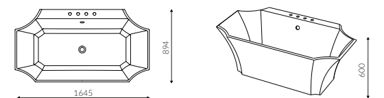
LA DONNA WANNA / BATHTUB
