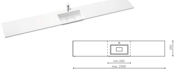
LIRA 2500 REGULOWANA / REGULATED
