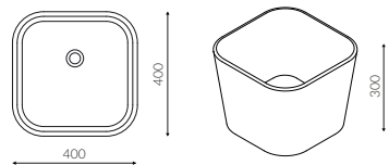
BALIA WANNA / BATHTUB
