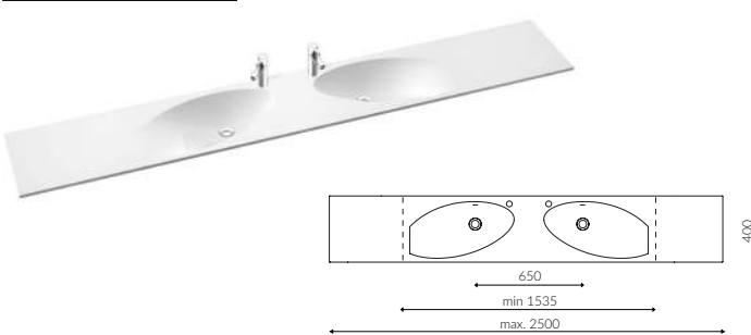
UGO DUET REGULOWANA / REGULATED
