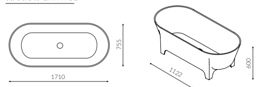
LIVA WANNA / BATHTUB
