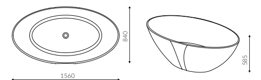
SELIA WANNA / BATHTUB
