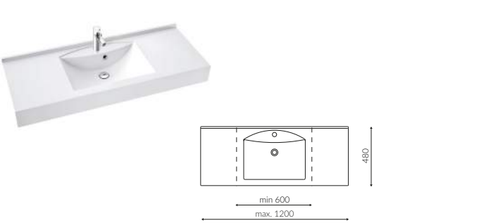
LARISSA HOTELOWA / HOTEL
