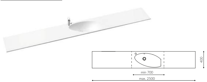
UGO 2500 REGULOWANA / REGULATED
