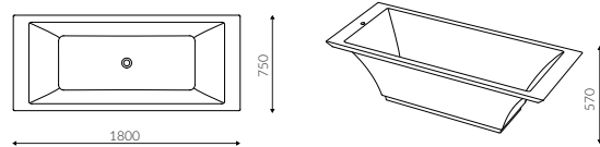
TEODOR WANNA / BATHTUB
