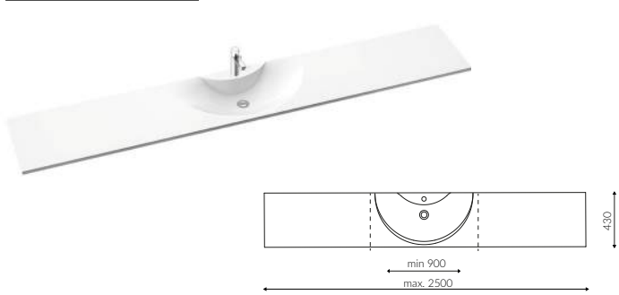
VERA 2500 REGULOWANA / REGULATED
